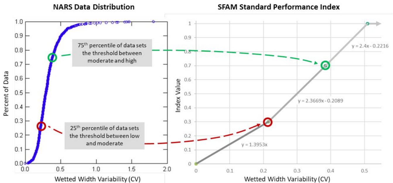
Figure 4.2 Raw Data Distributions from USEPA NARS Surveys are Used to Set Performance Expectations
