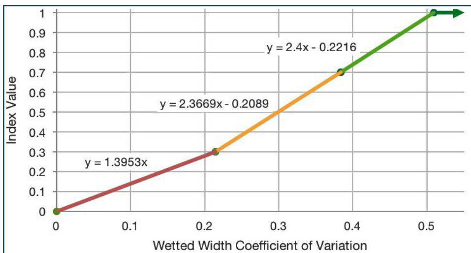
Figure 4.32 Wetted Width Standard Performance Index
