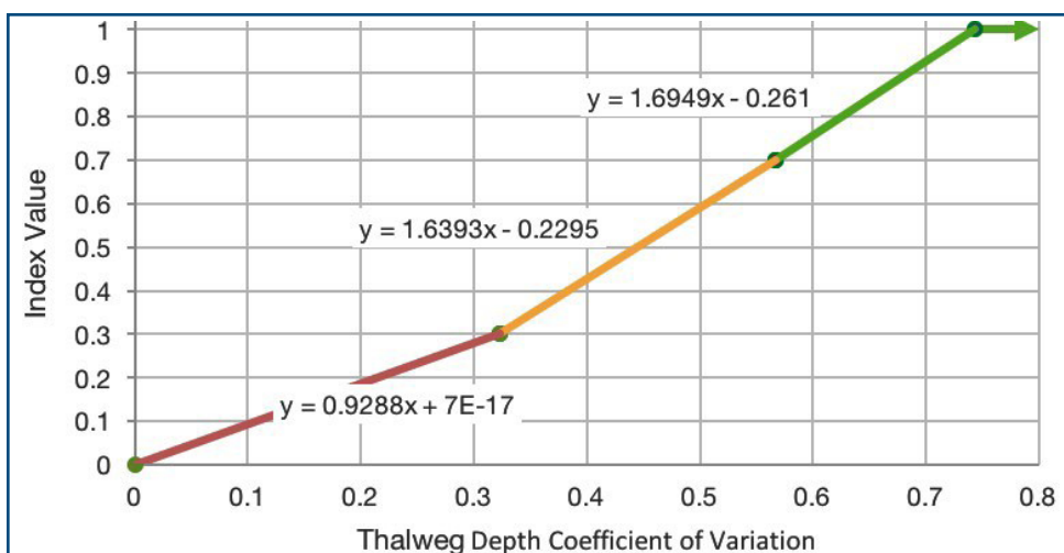
Figure 4.33 Thalweg Depth Standard Performance Index
