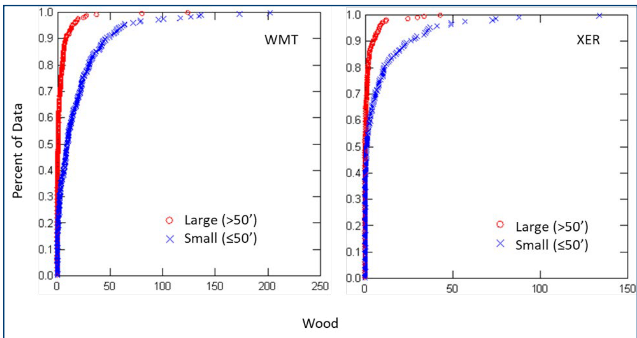
Figure 4.28 Frequency Distribution of Large Woody Debris Counts (per 328 feet) for 916 Stream Reaches by Size and Ecoregion
