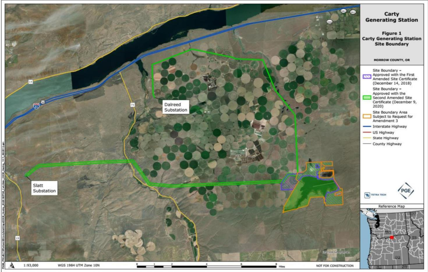
Figure 1: Approved Carty Generating Station Site Boundary and Vicinity
