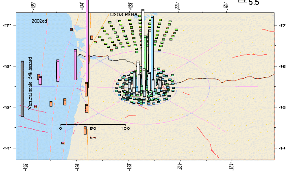
GMT 2004 Aug 23 12:07:02 Site Coords: 122.680 45.510 (yellow dot). Max annual ExceedRate: .1784E-03 (as lumin height prop. to ExRate). Red diamonds: historical earthquakes, Mw6
