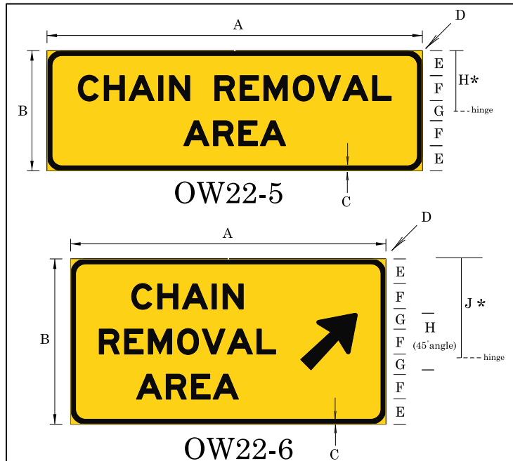
Figure 92: Sign OW22-5 & OW22-6 (CHAIN REMOVAL AREA) Detail
