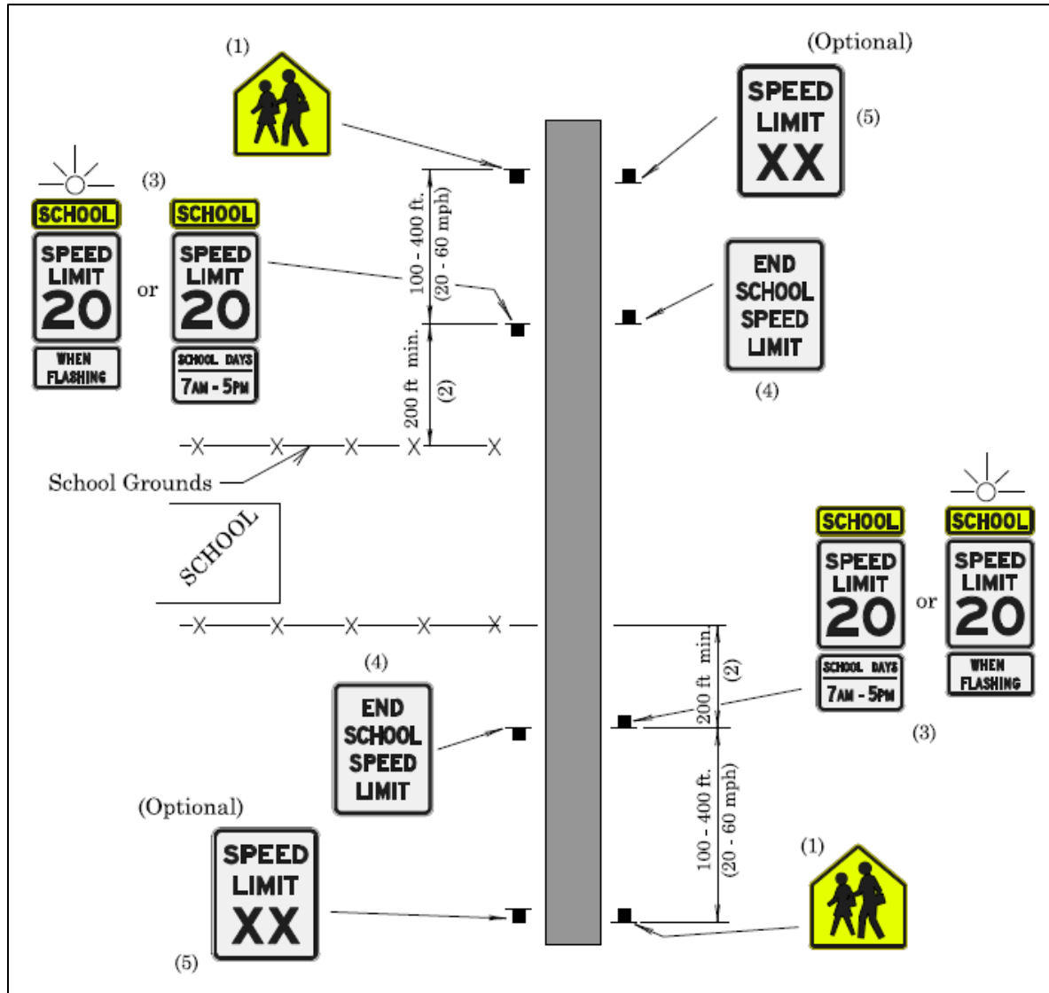
Figure 191: Condition "A" Layout without School Crosswalk
