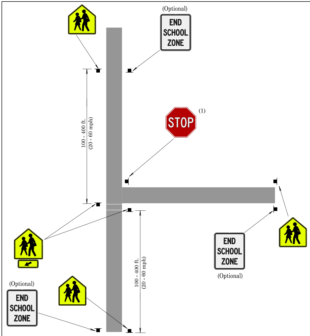
Figure 196: School Crosswalk Away From School (Optional)
