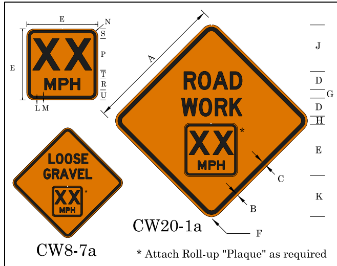
Figure 170: Signs CW20-1a & CW8-7a (ROAD WORK (LOOSE GRAVEL) XX MPH) Detail
