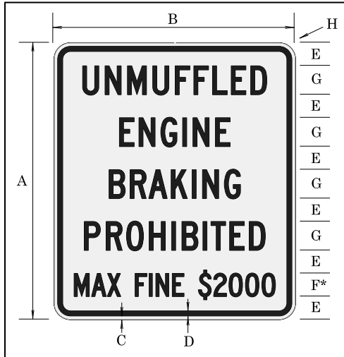
Figure 62: Sign OR22-11 (UNMUFFLED ENGINE BRAKING PROHIBITED) Detail
