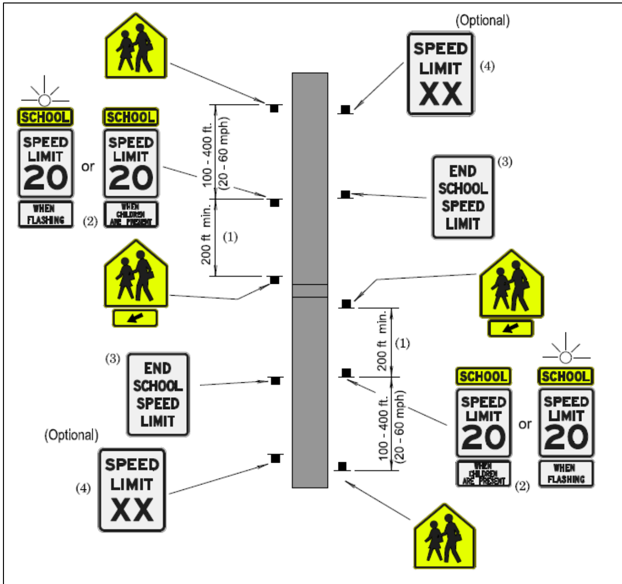
Figure 193: Condition "B" School Crosswalk Not Adjacent To School Grounds
