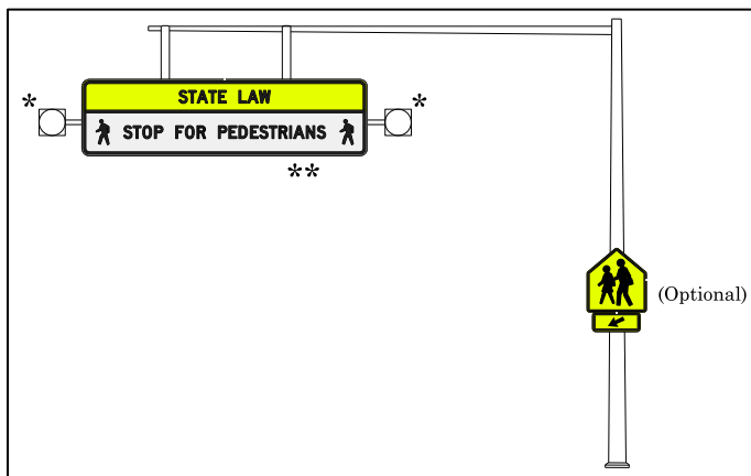
Figure 190: Ground-Mounted Overhead School Crossing Sign (Optional)
