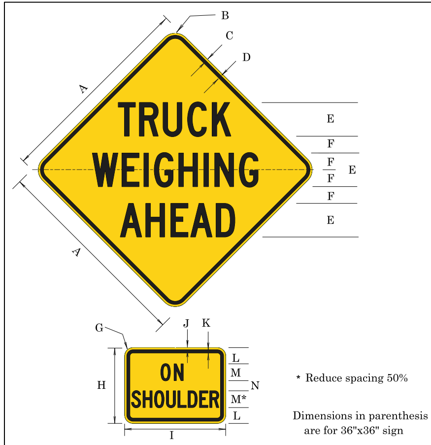
Figure 68: Sign OW7-5 (TRUCK WEIGHING AHEAD) Detail
