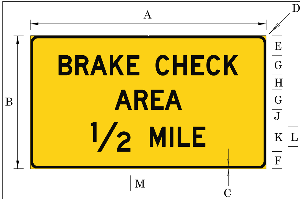
Figure 87: Sign OW21-4 (BRAKE CHECK AREA) Detail
