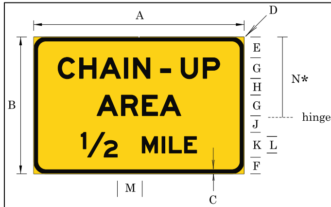
Figure 89: Sign OW22-1a (CHAIN-UP AREA) Detail
