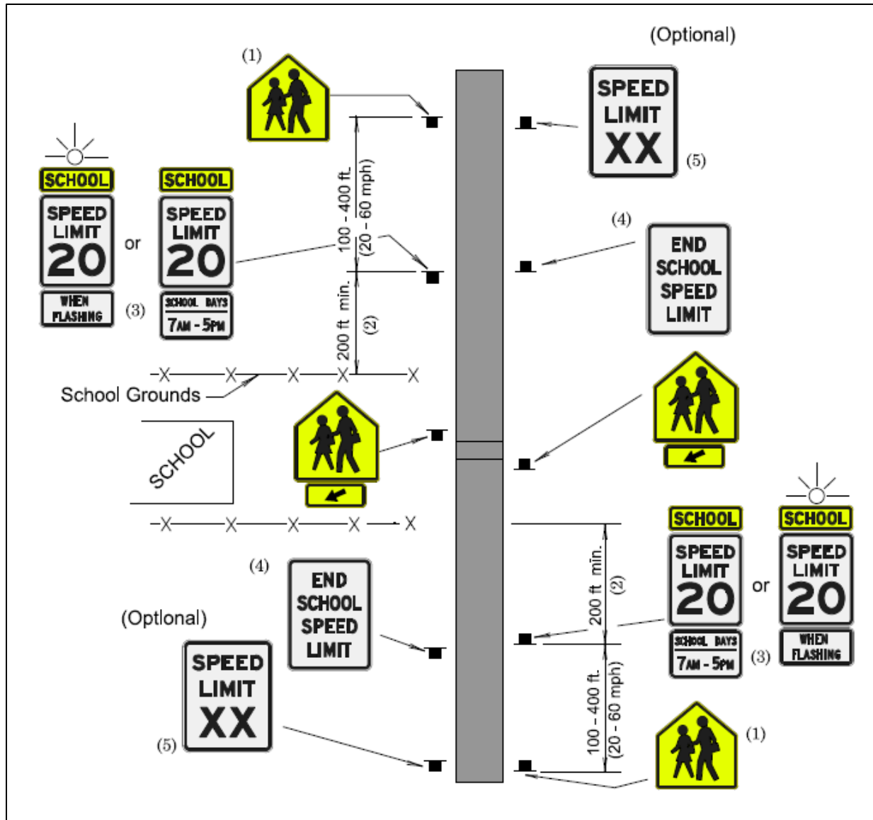
Figure 192: Condition "A" Layout with School Crosswalk
