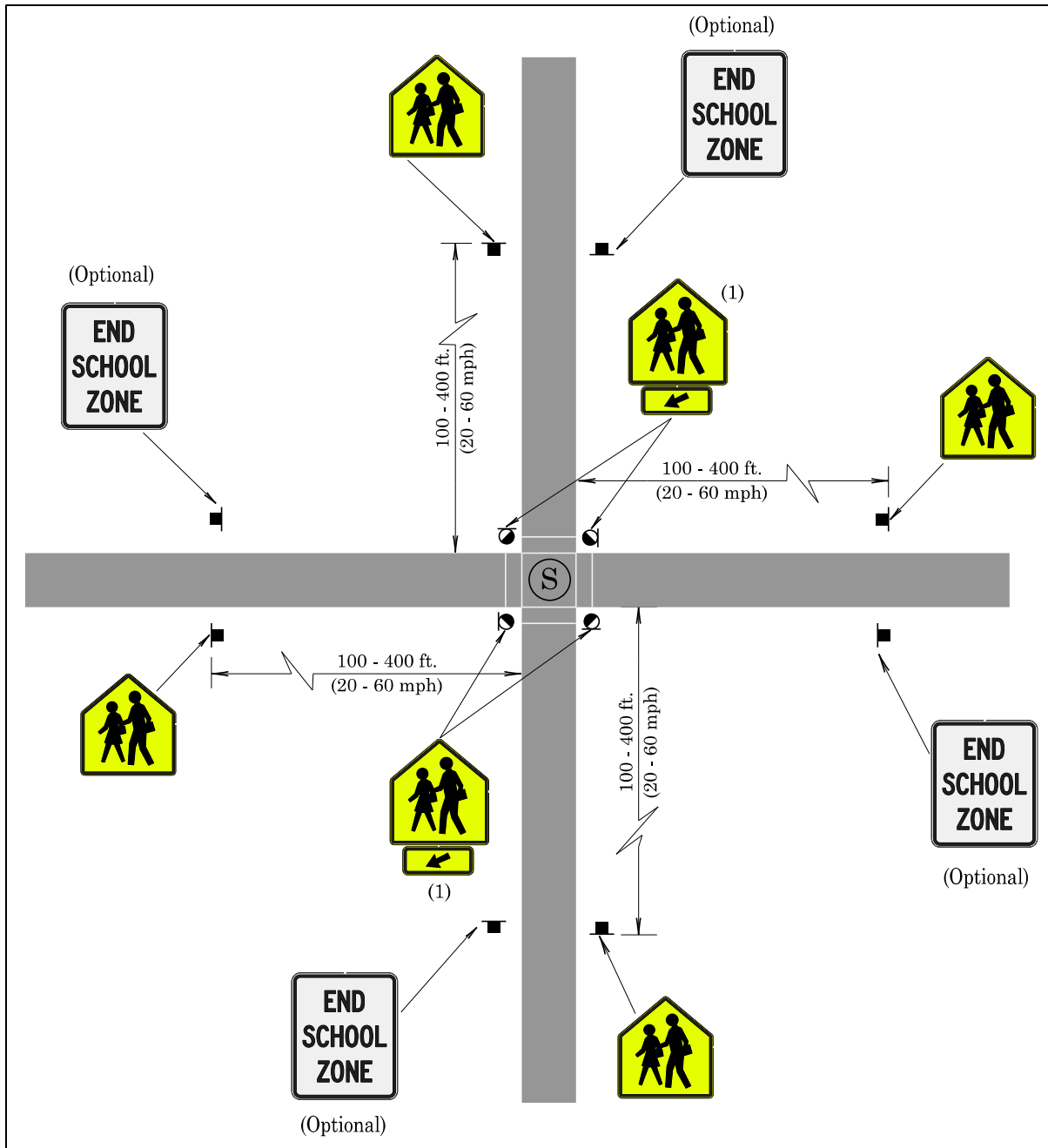
Figure 194: School Crosswalk Away From School at Signalized Intersection (Optional)
