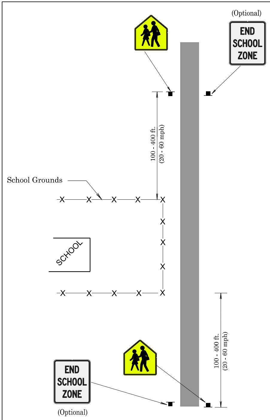
Figure 195: School Building Away From Highway or School Grounds Fenced (Optional)
