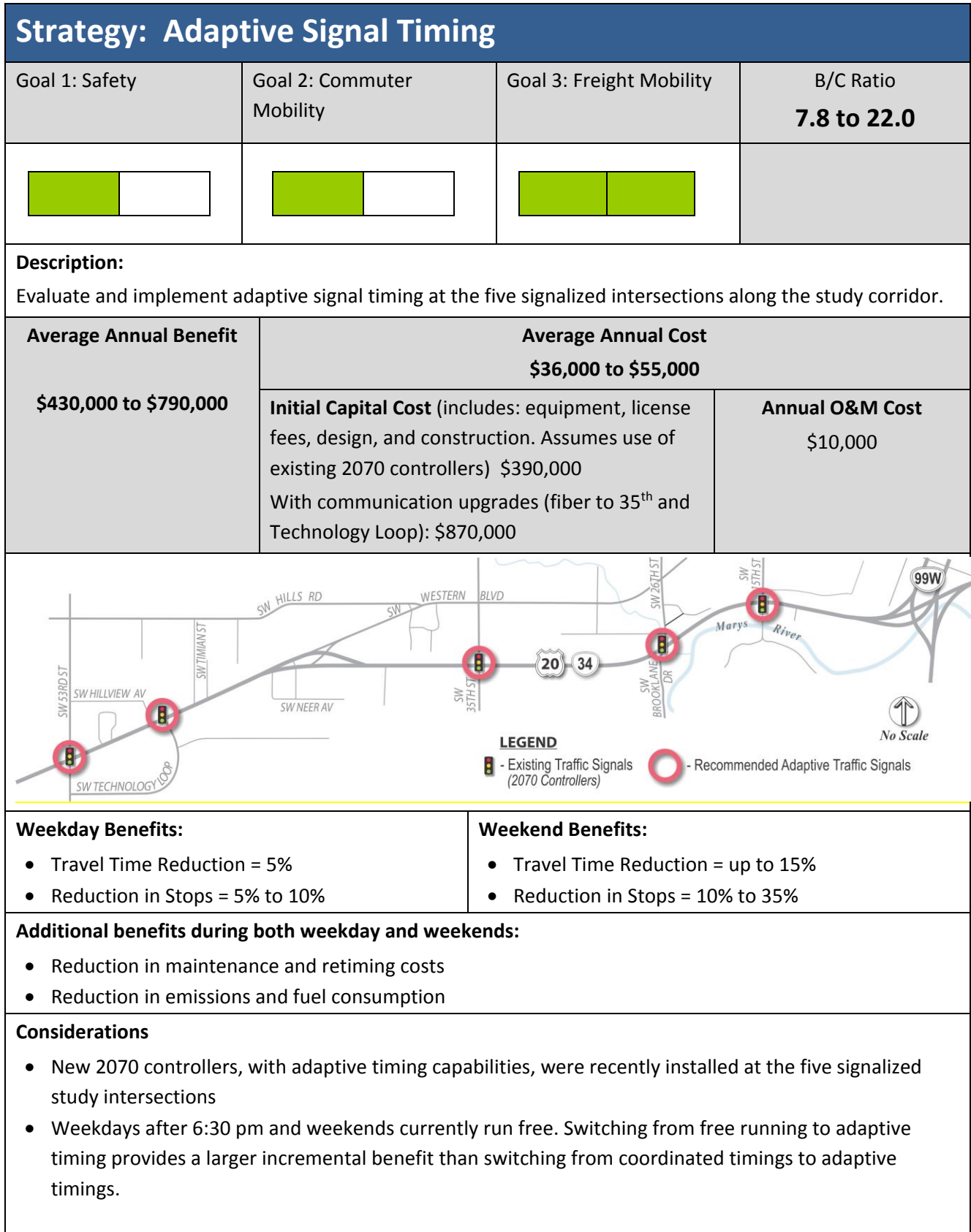
Figure 5-2: Adaptive Signal Timing
