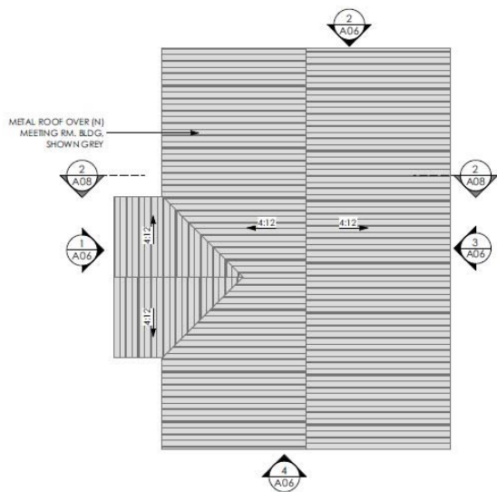
MEETING RM. PROPOSED ROOF PLAN SCALE: 1/8" = 1'-0" ②
