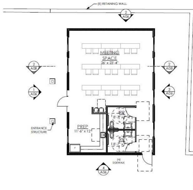
MEETING RM. PROPOSED FLOOR PLAN SCALE: 1/8" = 1'-0" ①
