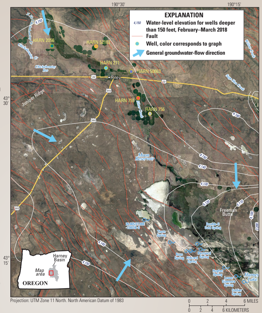
Locations of selected groundwater-level sites and groundwater-level contours (in feet above North American Vertical Datum of 1988) in the Silver Creek floodplain area, Harney Basin, southeastern Oregon. Contours from Gingerich and others, 2021. Background aerial image source: GoogleEarth™ 2019.
