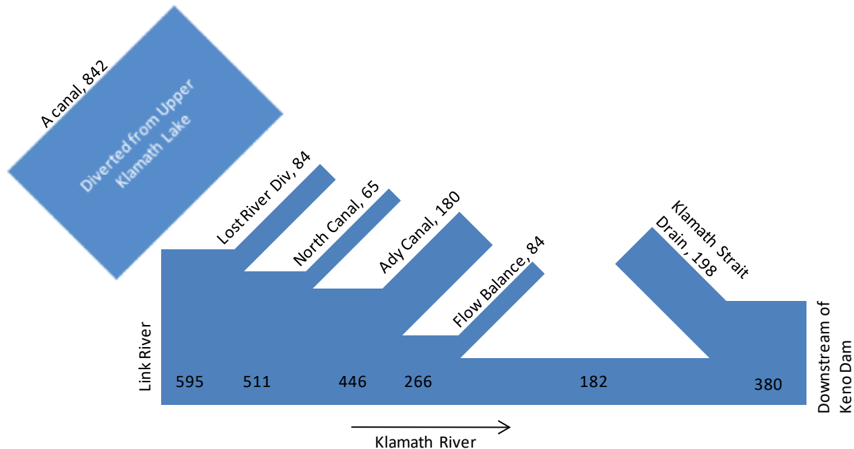
Figure 2-19. Schematic of an example flow balance in cubic feet per second for Keno impoundment (August 2002). Flows are represented by the thickness of each box.
