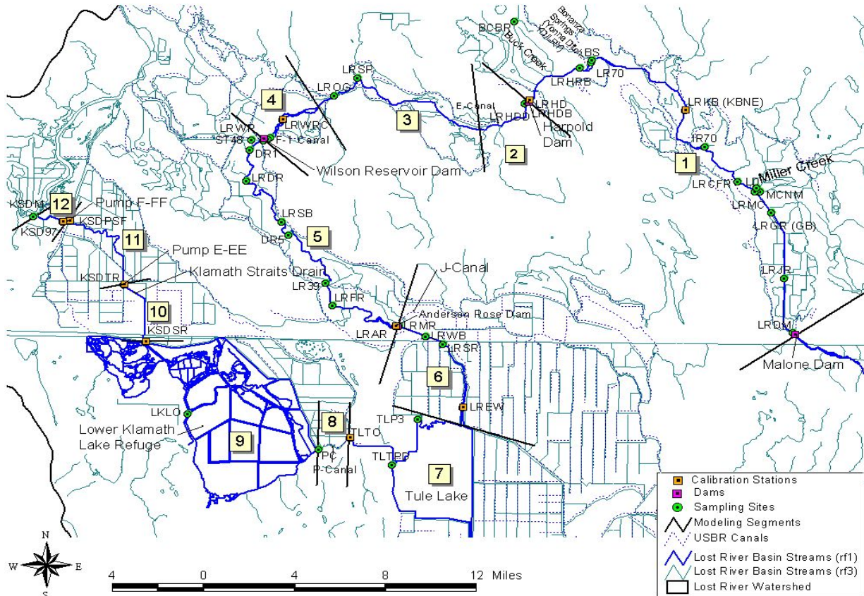
Figure 3-15. Model Configuration.
