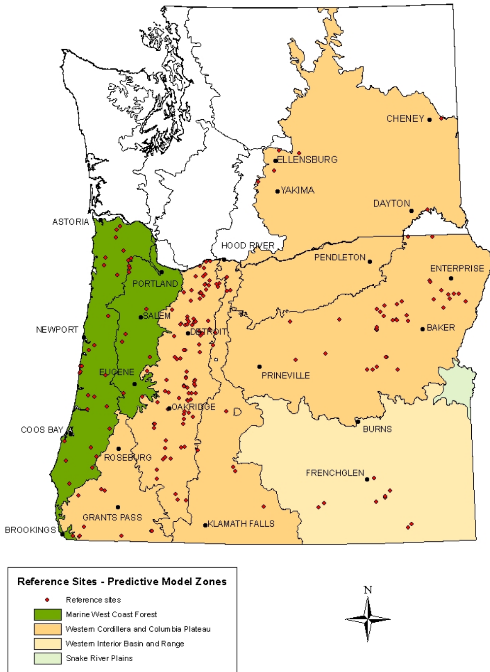
Figure 4. Map of PREDATOR reference sites and zones. PREDATOR consists of two predictive models (1-Marine West Coast Forest, 2-Western Cordillera and Columbia Plateau) and one null model (Western Interior Basin and Range). No model exists for the Snake River Plains ecoregion.
