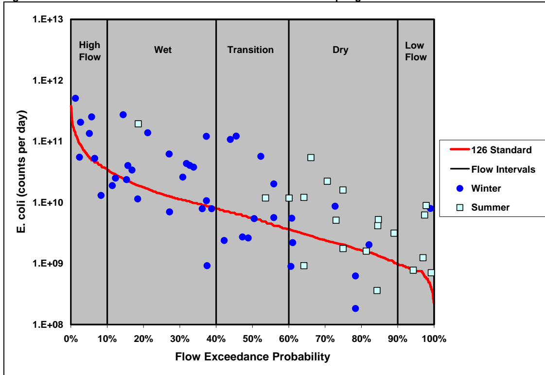
Figure 5.117. Load Duration Curve of Runoff and Non-Runoff Bacteria Loads in Springbrook Creek.
