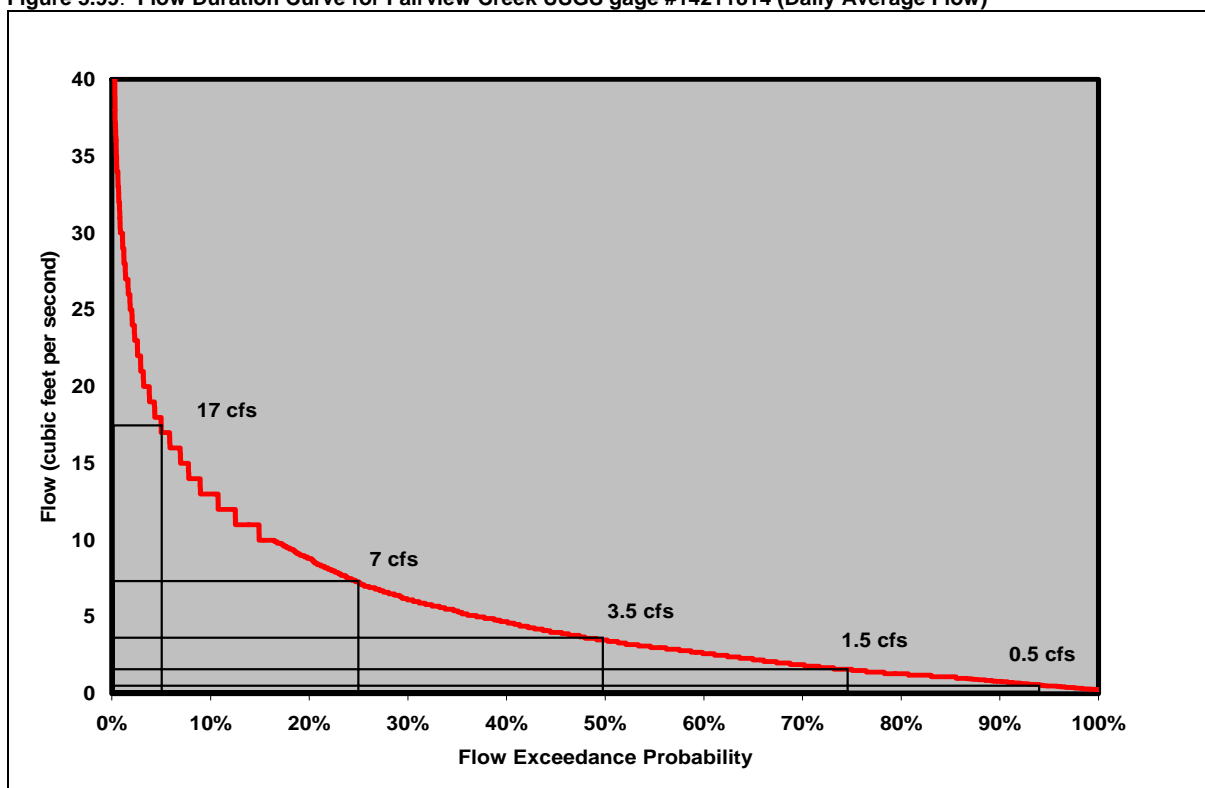
Figure 5.99. Flow Duration Curve for Fairview Creek USGS gage #14211814 (Daily Average Flow)
