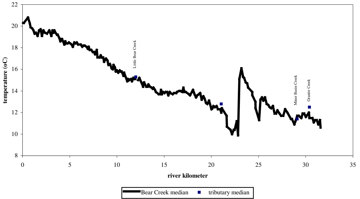
Appendix Figure A6. Longitudinal temperature profile of Bear Creek.
