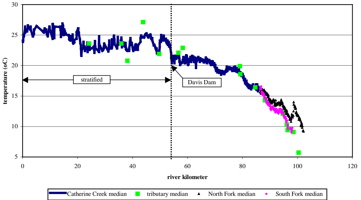
Appendix Figure A10. Longitudinal temperature profile of the Catherine Creek, North Fork and South Fork Catherine Creek.
