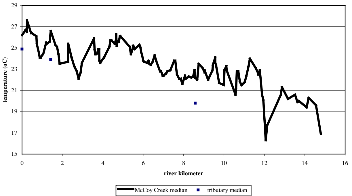
Appendix Figure A13. Longitudinal temperature profile of McCoy Creek.
