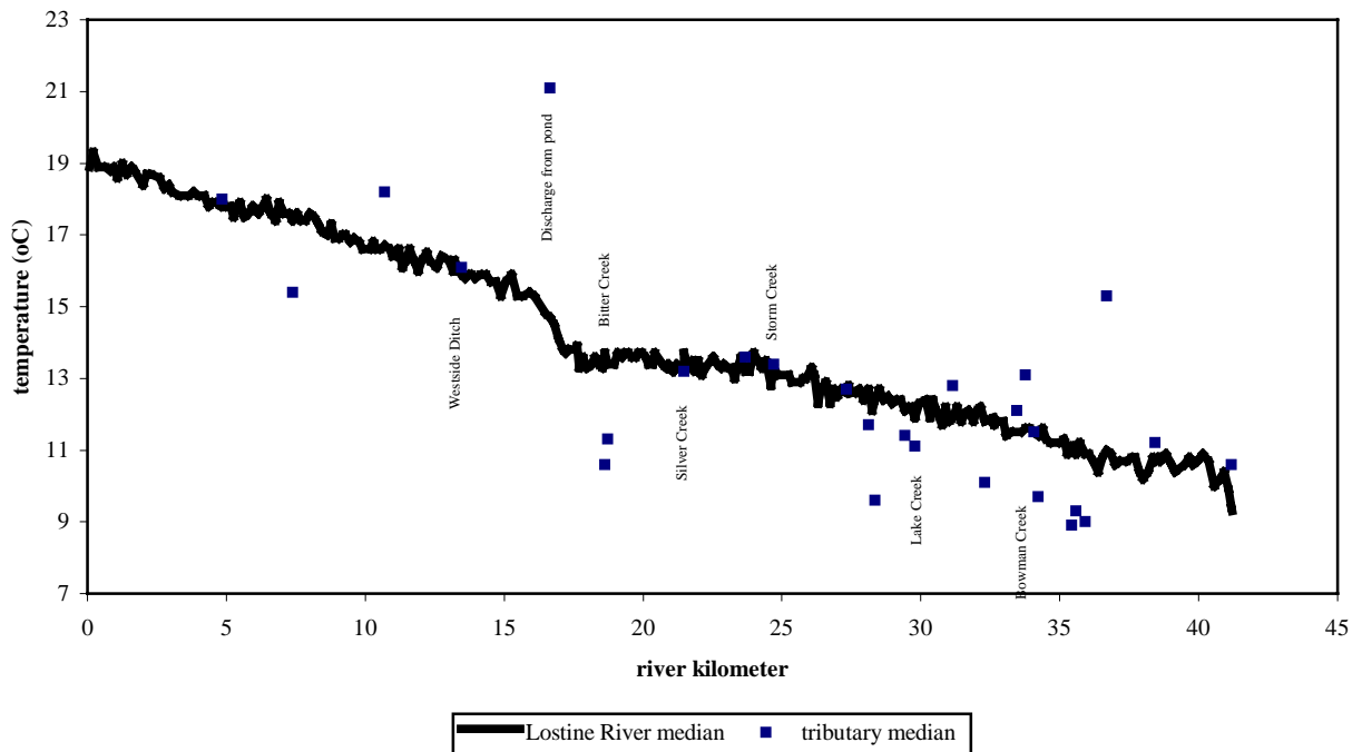
Appendix Figure A5. Longitudinal temperature profile of the Lostine River.
