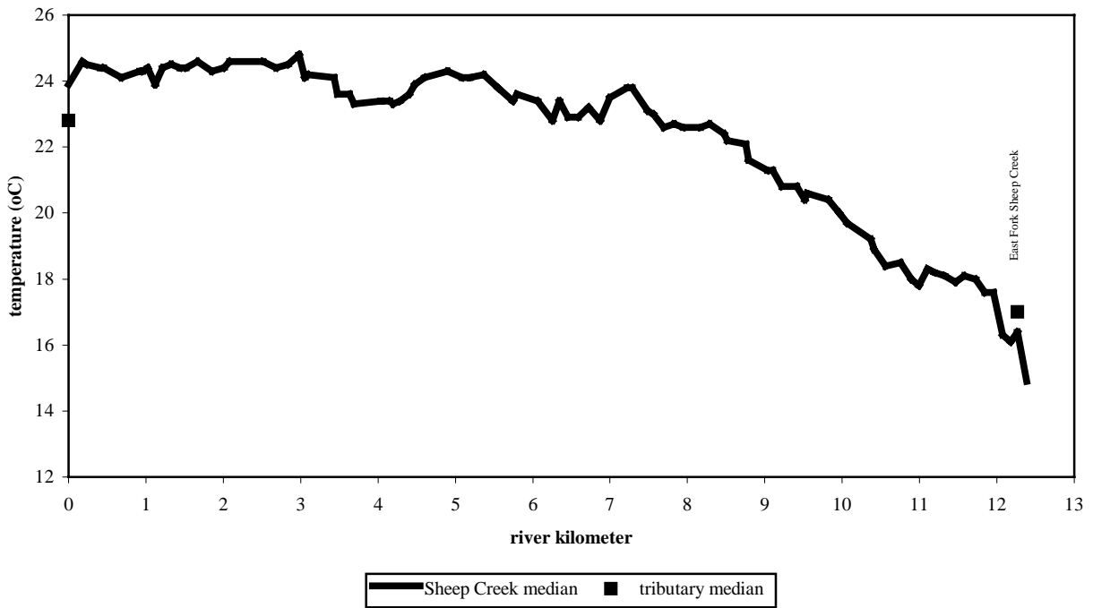
Appendix Figure A15. Longitudinal temperature profile of Sheep Creek.
