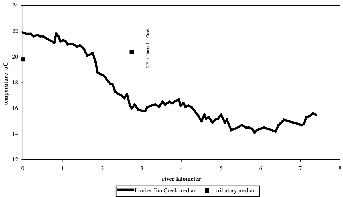
Appendix Figure A16. Longitudinal temperature profile of Limber Jim Creek.
