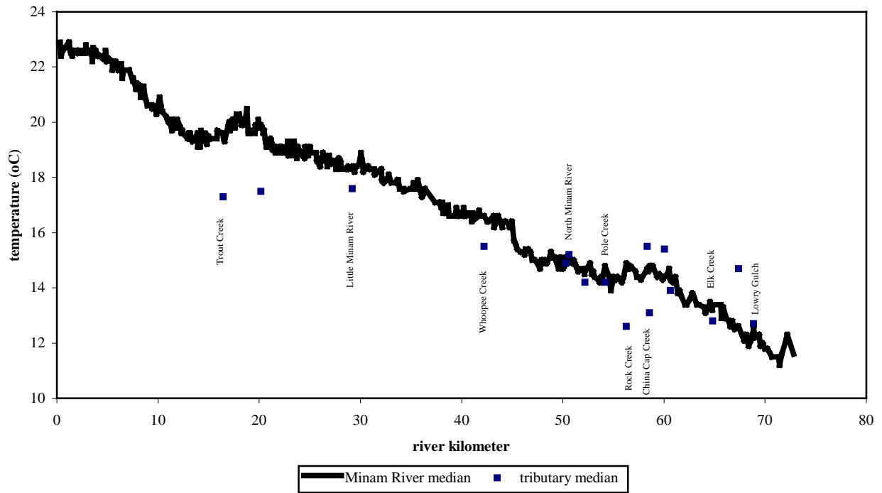
Appendix Figure A4. Longitudinal temperature profile of the Minam River.
