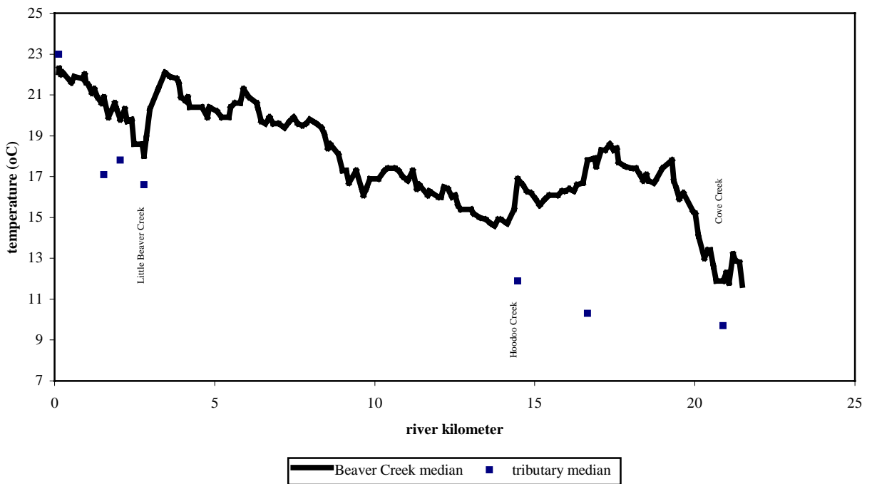
Appendix Figure A11. Longitudinal temperature profile of Beaver Creek.
