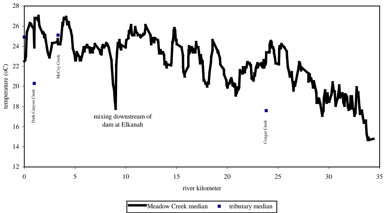
Appendix Figure A12. Longitudinal temperature profile of Meadow Creek.
