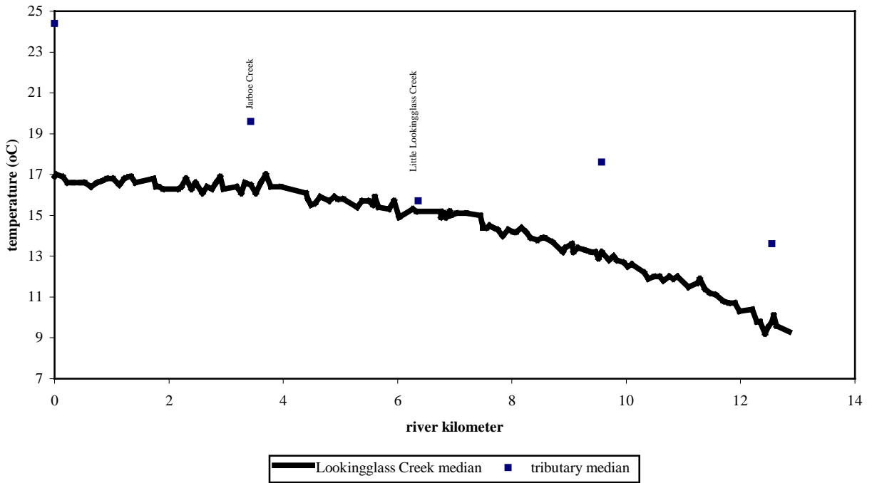
Appendix Figure A7. Longitudinal temperature profile of Lookingglass Creek.
